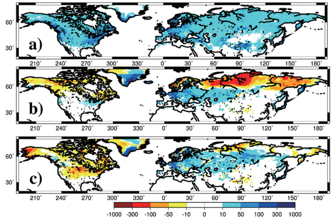
Figure 1. Difference between 1986–1995 mean annual snowfall (mm/year) as computed with a) 0°C threshold method, b) LW90 and c) Ad03, and H08 snowfall.
