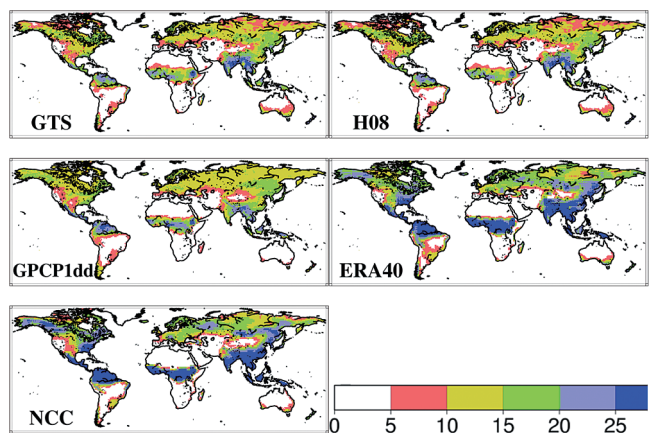
Figure 2. 1986–1995 mean number of precipitation days (days with precipitation > 0.5 mm/day) in July.
