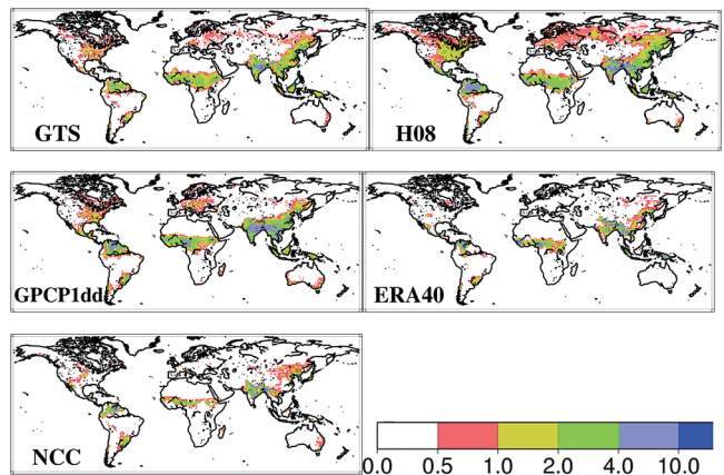
Figure 3. 1986–1995 mean number of heavy precipitation days (days with precipitation > 20 mm/day) in July.
