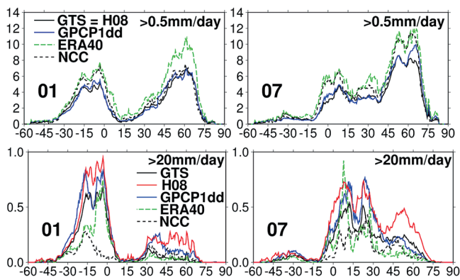
Figure 1. Zonal means of number of precipitation days (> 0.5 mm/day) (top) and of number of heavy precipitation days (> 20 mm/day) (bottom) for January (left) and July (right). All values are means from 1986 to 1995.
