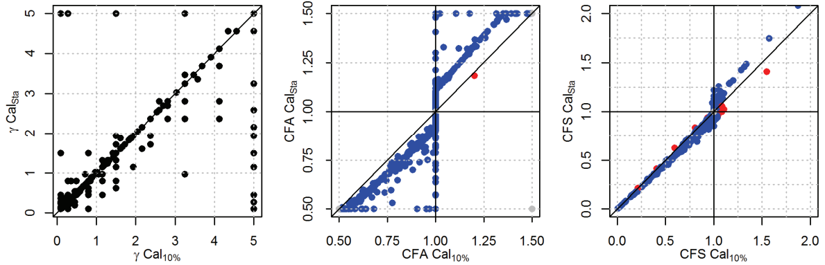
Fig. A7: Scatter plots of calibration parameters \gamma (left), CFA (center) and CFS (right) for calibration considering ( \text{Cal}_{10\%} ) and not considering ( \text{Cal}_{\text{Sta}} ) 10% uncertainty in observed river discharge. Blue colors for CFA and CFS indicate basins with a value closer to unity, and red colors the opposite. Grey colors (CFA) indicate no changes in the parameter value. Horizontal and vertical lines for CFA and CFS indicate the value of unity, whereas the diagonal line in all three plots shows the 1:1 line.
