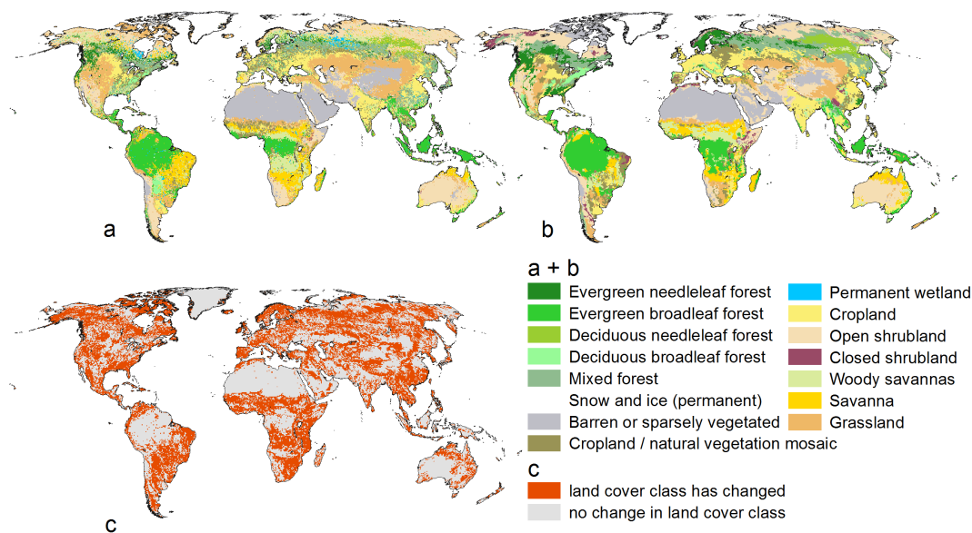
Figure 2. Land cover maps with a spatial resolution of 0.5° used as WaterGAP input based on MODIS observations for the year 2004 (variant STANDARD) (a), land cover derived from USGS GLCC, but CORINE for Europe, reflecting land cover distribution around the year 2000 (variant LANDCOVER) (b), and identification of grid cells where land cover class has changed due to different input data (c).
