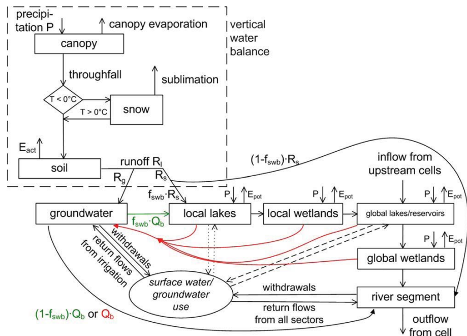
Figure 1. Schematic of water storage compartments (boxes) and flows (arrows) within each 0.5^\circ grid cell of the WaterGAP Global Hydrology Model, including the simulation of water use impacts on water storage in groundwater and surface water. Compared to WaterGAP 2.1h [Döll et al., 2012, Figure 1], routing of surface runoff and base flow was modified to simulate that not the whole runoff from land R_l is routed through the surface water bodies. In addition, in semiarid and arid regions, groundwater recharge is assumed to occur beneath surface water bodies (lakes, wetlands, and reservoirs but not rivers), while in humid areas, groundwater recharges surface water bodies. Flows that are only modeled in semiarid and arid regions are shown in red and those occurring only in humid regions are shown in green.
