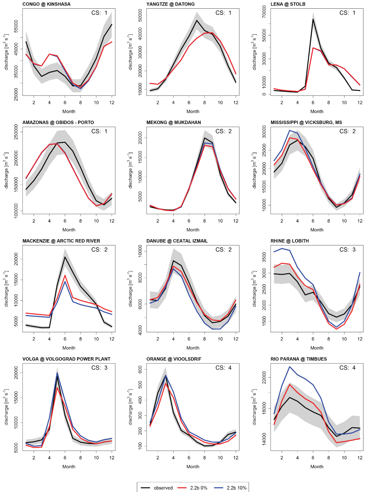
Fig. A8: Observed and simulated discharge seasonality of WaterGAP 2.2b runs with \text{Cal}_{10\%} (blue color), \text{Cal}_{\text{Sta}} (red) and observed values (black) including a 10% variation of mean monthly values (grey) and an indicator of calibration status (CS; see Sect. A3.2) for the large river basins that were used in Müller Schmied et al. (2014).
